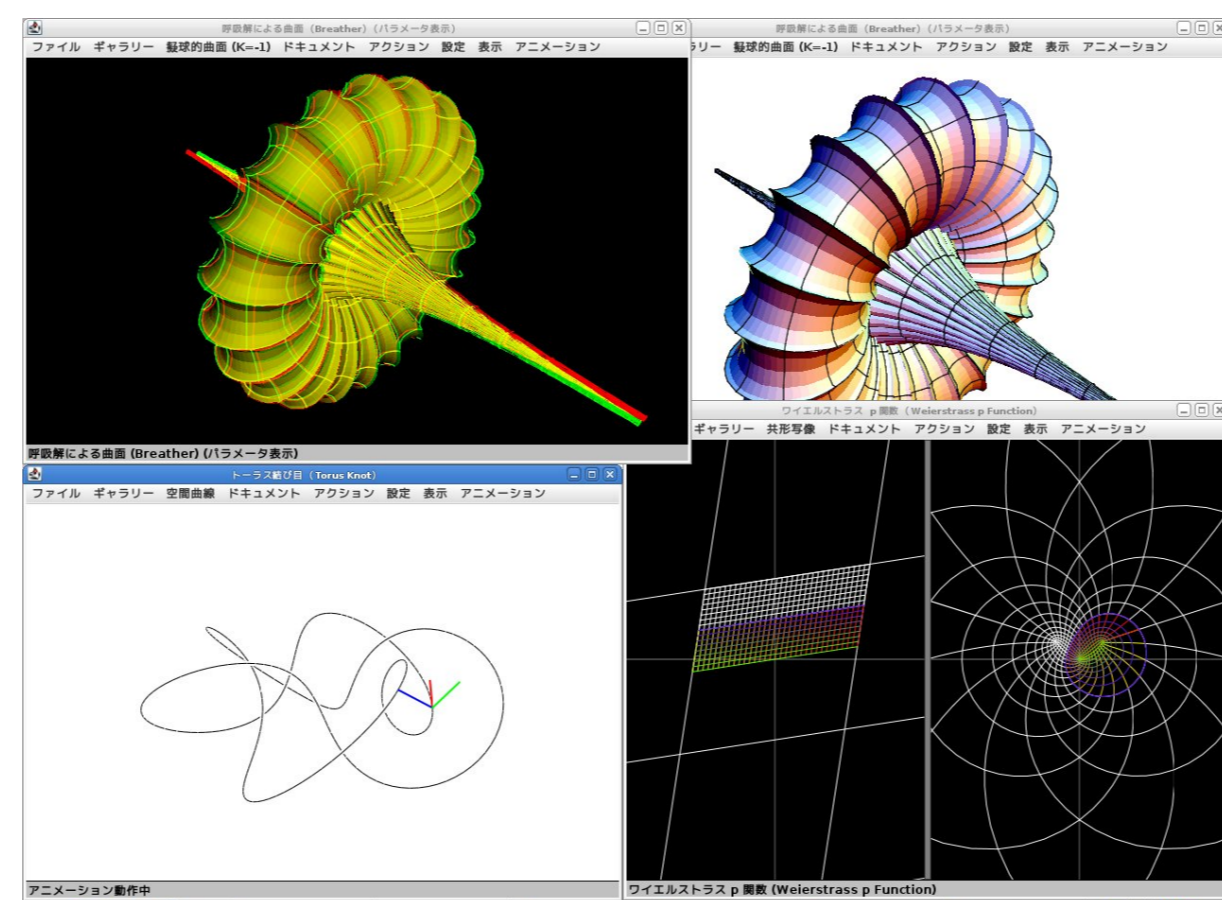
Figure 4: 3D-XplorMath-J
