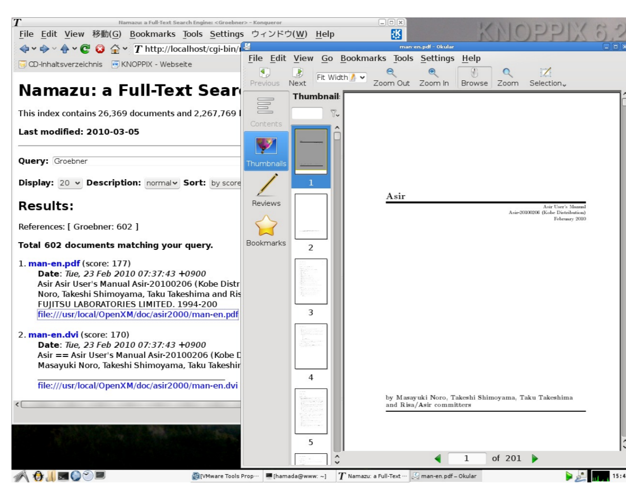
Figure 3: MathDoc-Search
