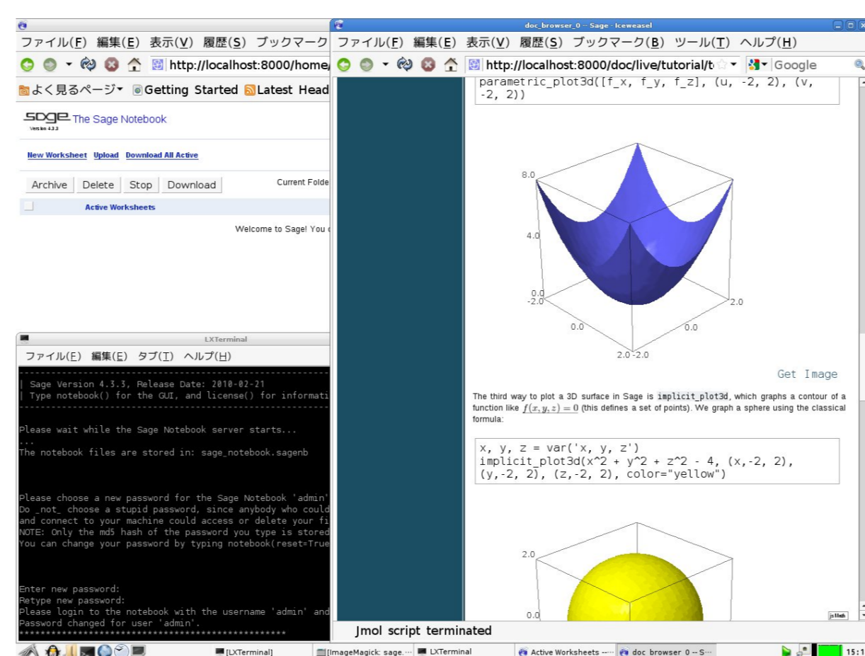
Figure 9: SAGE notebook
