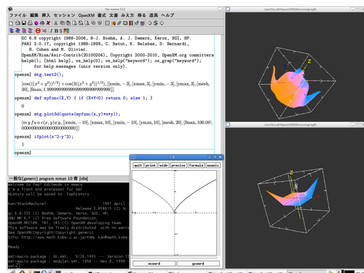
Figure 7: Risa/Asir(OpenXM)
