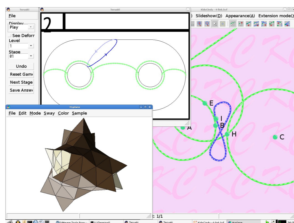
Figure 5: AharaLab
