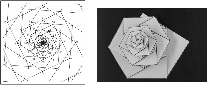
Fig. 1 A spiral multiple tiling by right triangles with angles 30^\circ , 60^\circ , 90^\circ and top-down view.
