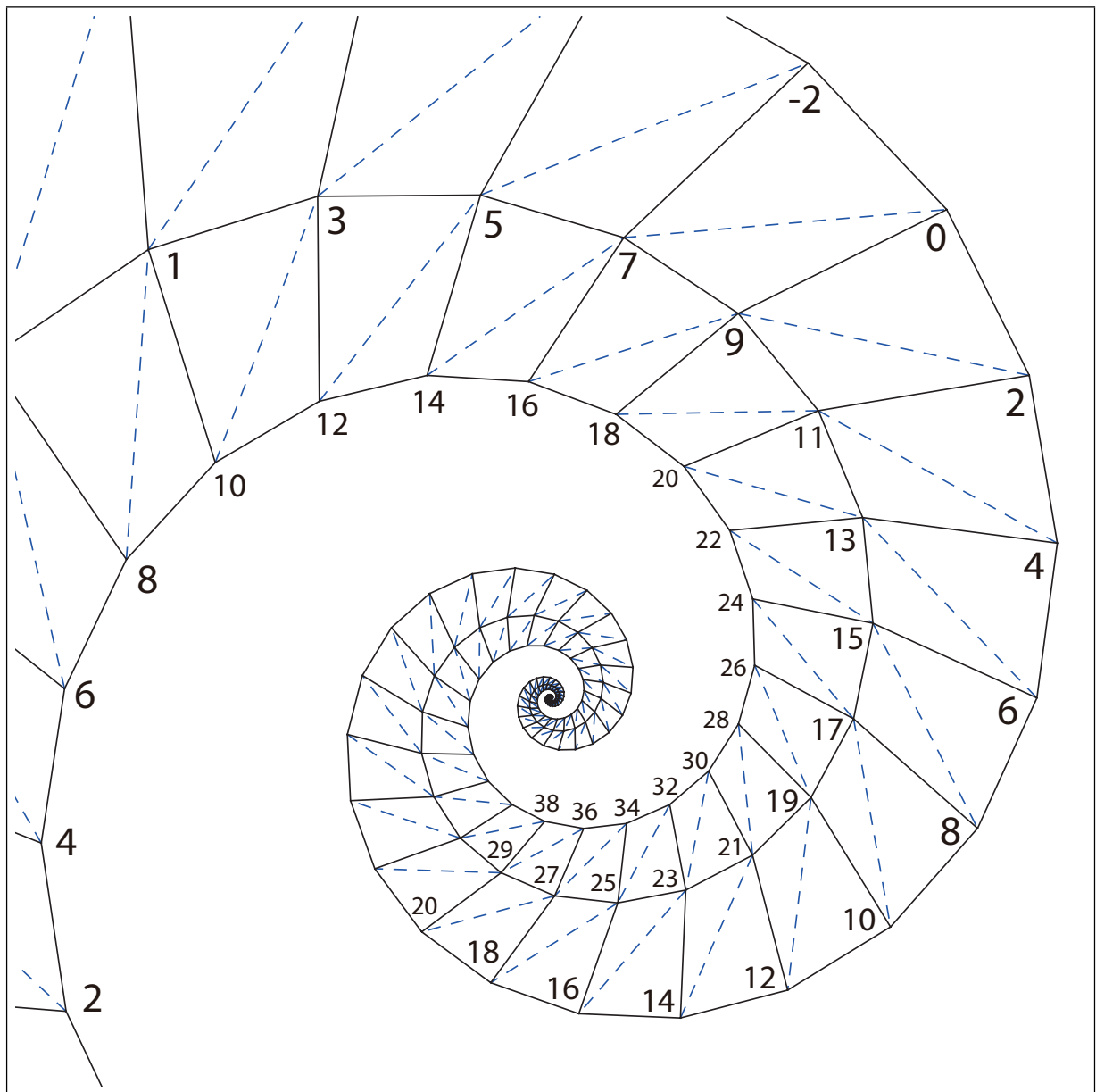
Fig. 2 An origami sheet for a spiral multiple tiling by right triangles with angles 30^\circ , 60^\circ , 90^\circ : Blue dashed lines are valley fold and black solid lines are mountain fold.
