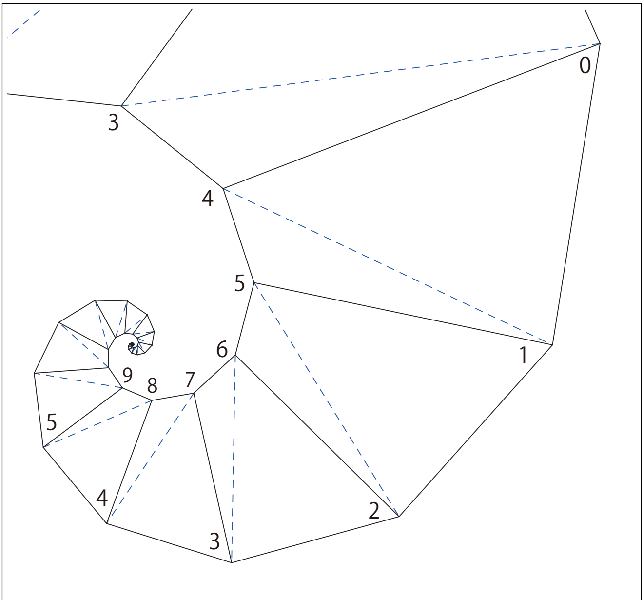
Fig. 2 An origami sheet for a spiral tiling by regular triangles : Blue dashed lines are valley fold and black solid lines are mountain fold.
